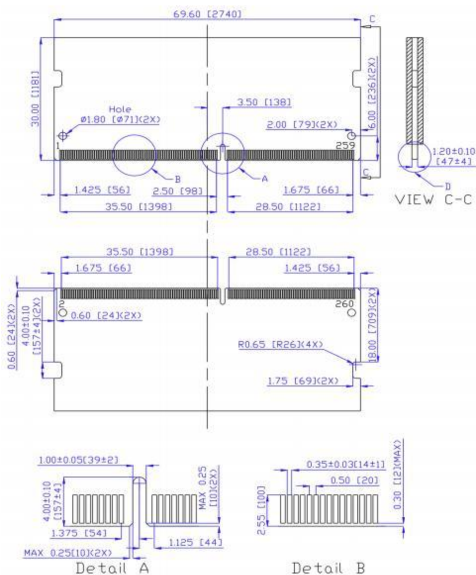
Figure 4 Module Dimension
