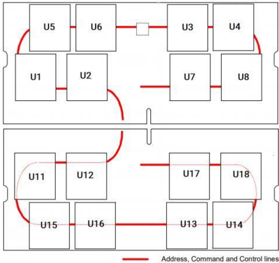
Figure 3 Functional Diagram(II)
