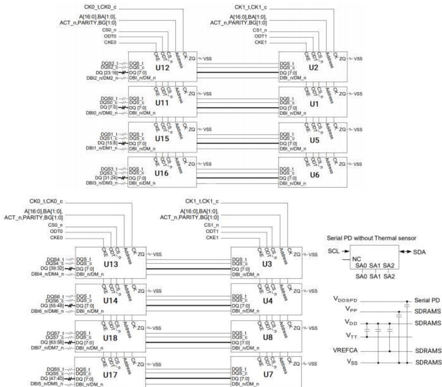
Figure 2 Functional Diagram( I )
