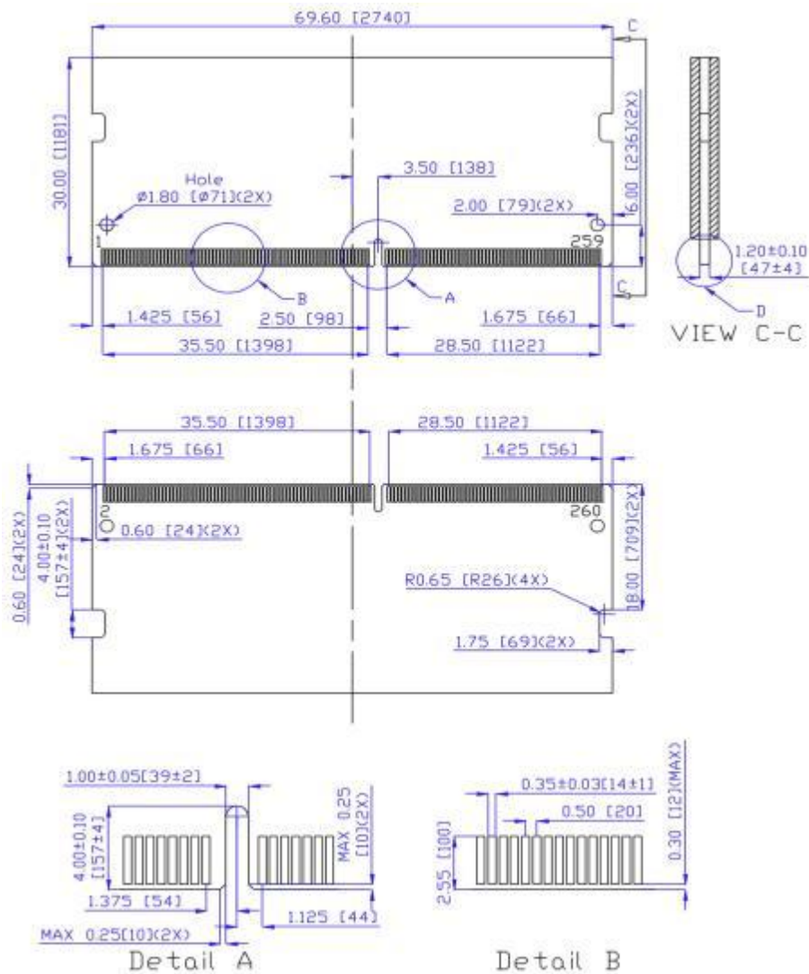
Figure 3 Module Dimension
